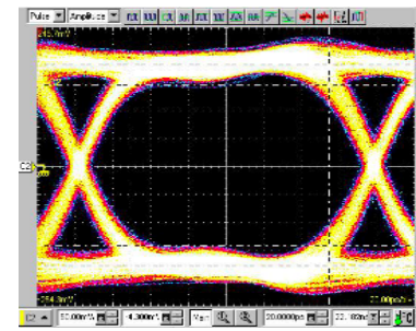
3EH-2A16J with Fixture: pin#5-pin#8 Rise Time: \approx 30\text{ps} , Bit Rate: 6.4Gb/s PRBS (Pseudo Random Bit Sequence): 2^{10}-1
