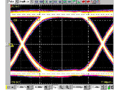
3EH-2A16J with Fixture: pin#5-pin#8 Rise Time: \approx 250\text{ps} , Bit Rate: 1.6Gb/s PRBS (Pseudo Random Bit Sequence): 2^{10}-1
