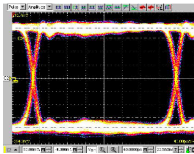
Through Fixture Rise Time: \approx 30\text{ps} , Bit Rate: 3.2Gb/s PRBS (Pseudo Random Bit Sequence): 2^{10}-1
