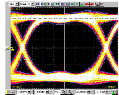
3EH-2A16J with Fixture: pin#3-pin#10 Rise Time: \approx 30\text{ps} , Bit Rate: 6.4Gb/s PRBS (Pseudo Random Bit Sequence): 2^{10}-1
