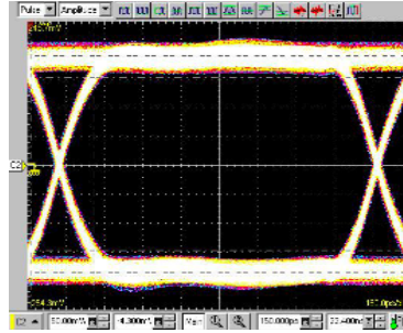
3EH-2A16J with Fixture: pin#3-pin#10 Rise Time: \approx 250\text{ps} , Bit Rate: 800Mb/s PRBS (Pseudo Random Bit Sequence): 2^{10}-1
