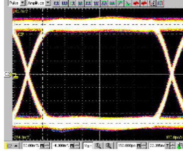
3EH-2A16J with Fixture: pin#5-pin#8 Rise Time: \approx 250\text{ps} , Bit Rate: 800Mb/s PRBS (Pseudo Random Bit Sequence): 2^{10}-1
