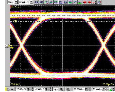
3EH-2A16J with Fixture: pin#3-pin#10 Rise Time: \approx 250\text{ps} , Bit Rate: 1.6Gb/s PRBS (Pseudo Random Bit Sequence): 2^{10}-1
