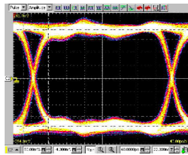
3EH-2A16J with Fixture: pin#5-pin#8 Rise Time: \approx 30\text{ps} , Bit Rate: 3.2Gb/s PRBS (Pseudo Random Bit Sequence): 2^{10}-1
