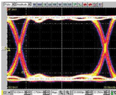
Through Fixture Rise Time: \approx 30 ps, Bit Rate: 6.4Gb/s PRBS (Pseudo Random Bit Sequence): 2^{10}-1
