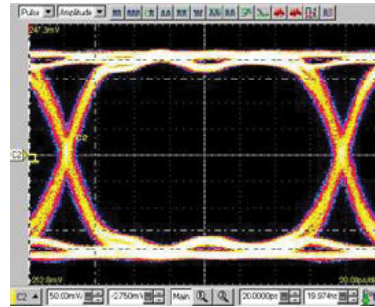
1EH-16A with Fixture Rise Time: \approx 30 ps, Bit Rate: 6.4Gb/s PRBS (Pseudo Random Bit Sequence): 2^{10}-1
