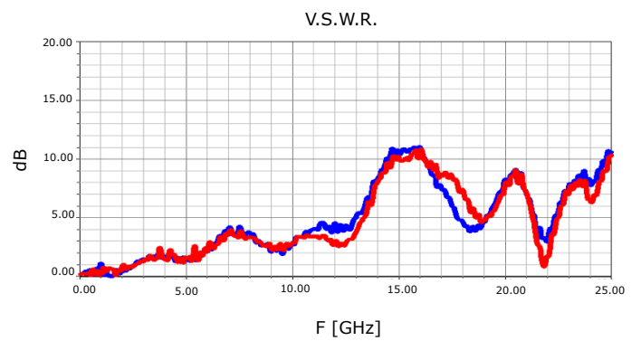
1EH-16A with Fixture Rise Time: \approx 30 ps, Bit Rate: 6.4Gb/s PRBS (Pseudo Random Bit Sequence): 2^{10}-1
