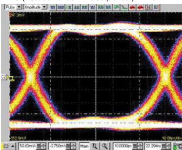
Through Fixture Rise Time: \approx 30 ps, Bit Rate: 12.8Gb/s PRBS (Pseudo Random Bit Sequence): 2^{10}-1
