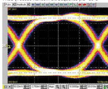
1EH-16A with Fixture Rise Time: \approx 30 ps, Bit Rate: 12.8Gb/s PRBS (Pseudo Random Bit Sequence): 2^{10}-1
