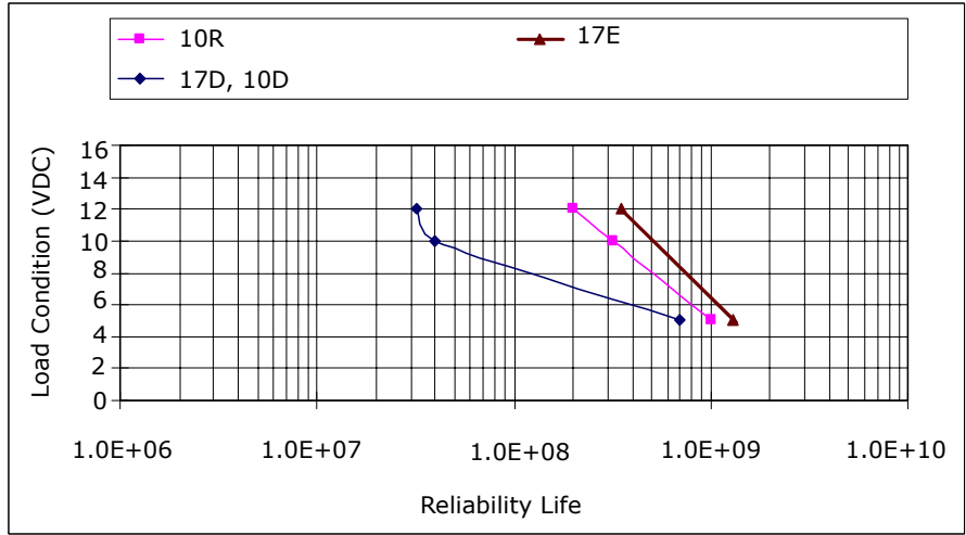
Reliability and load condition (100mW) Data
