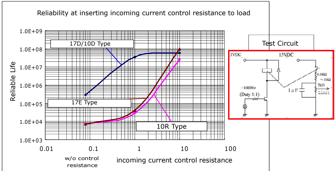
Reliability Vs. Capacitive load data (Load condition 15V 2kΩ 1μF)
